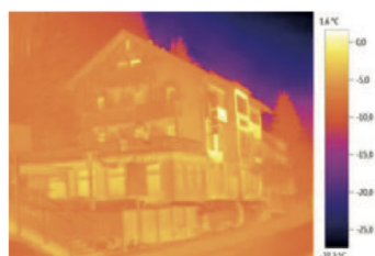
Thermal image without ScaleAssist
